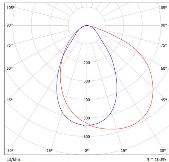
cd/klm ..... \eta = 100\%
